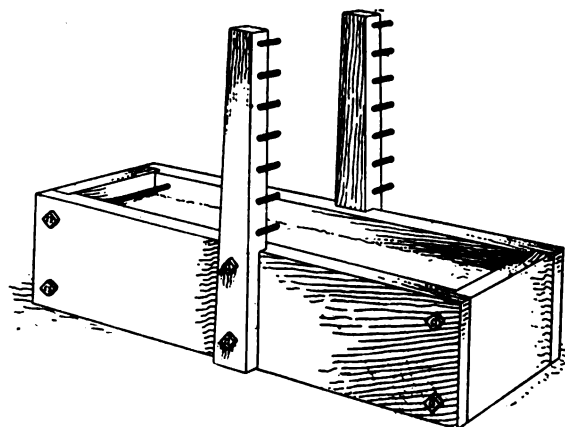
Fig. 2—The wheel trough used in conjunction with gas heater for heating tires
